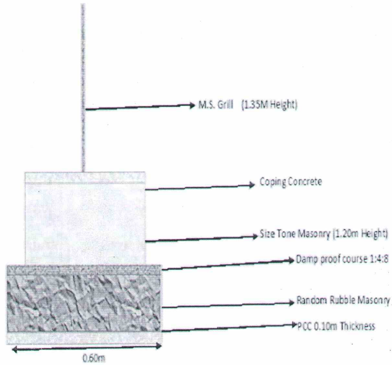
Section of boundary wall
